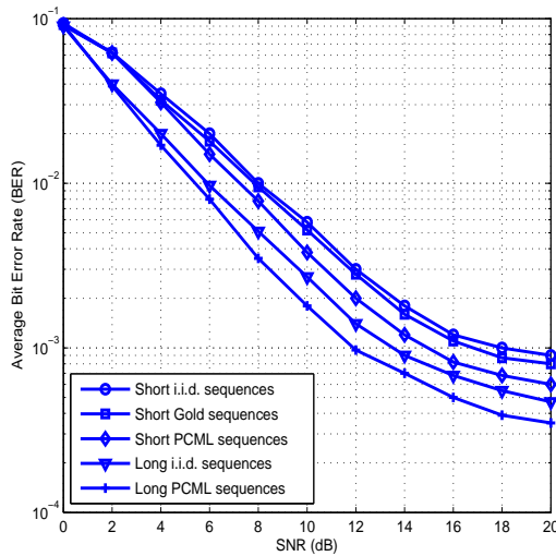
Fig. 9. Average BER versus SNR for 2^{th} order monocyce assuming 15 asynchronous interferers.
