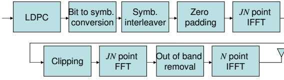
Fig. 4. Transmitter
