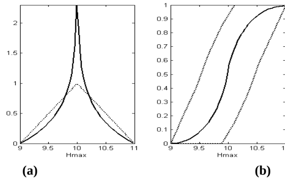
Figure 3: (a) Possibilistic distribution of H_{max} (dotted line) and its probabilistic transformation (continuous line); (b) corresponding necessity and possibility measures of the set (-\infty, H_{max}] (dotted line) and cumulative distribution function of H_{max} considered by the purely probabilistic method (continuous line).
