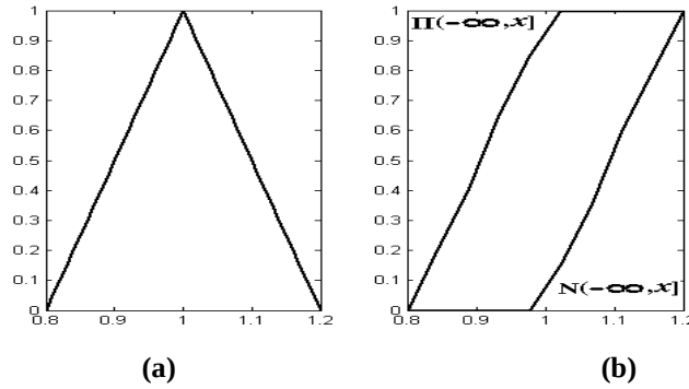
Figure 1: Example of: (a) triangular possibilistic distribution and (b) corresponding possibility and necessity measures of the set A = (-\infty, x]
