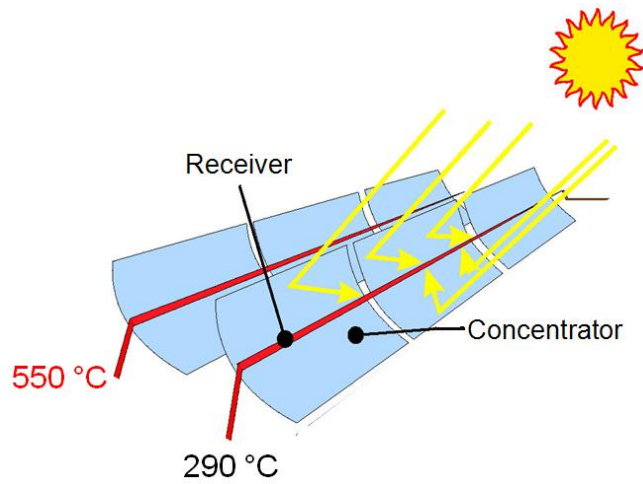
Figure 1: scheme of the X-ITE through parabolic collector solar plant
