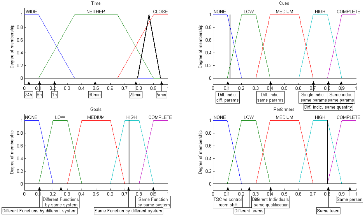
Figure 18. Fuzzy input with trapezoidal MFs for case 3: range assessment.
