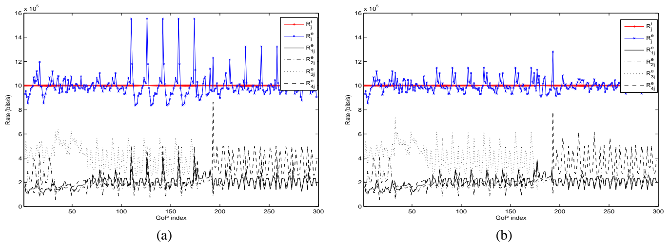
Figure 4. Evolution of the total transmission rates as well as individual and total encoding rates for the four multiplexed programs when W = 2 (a) and W = 4 (b)
