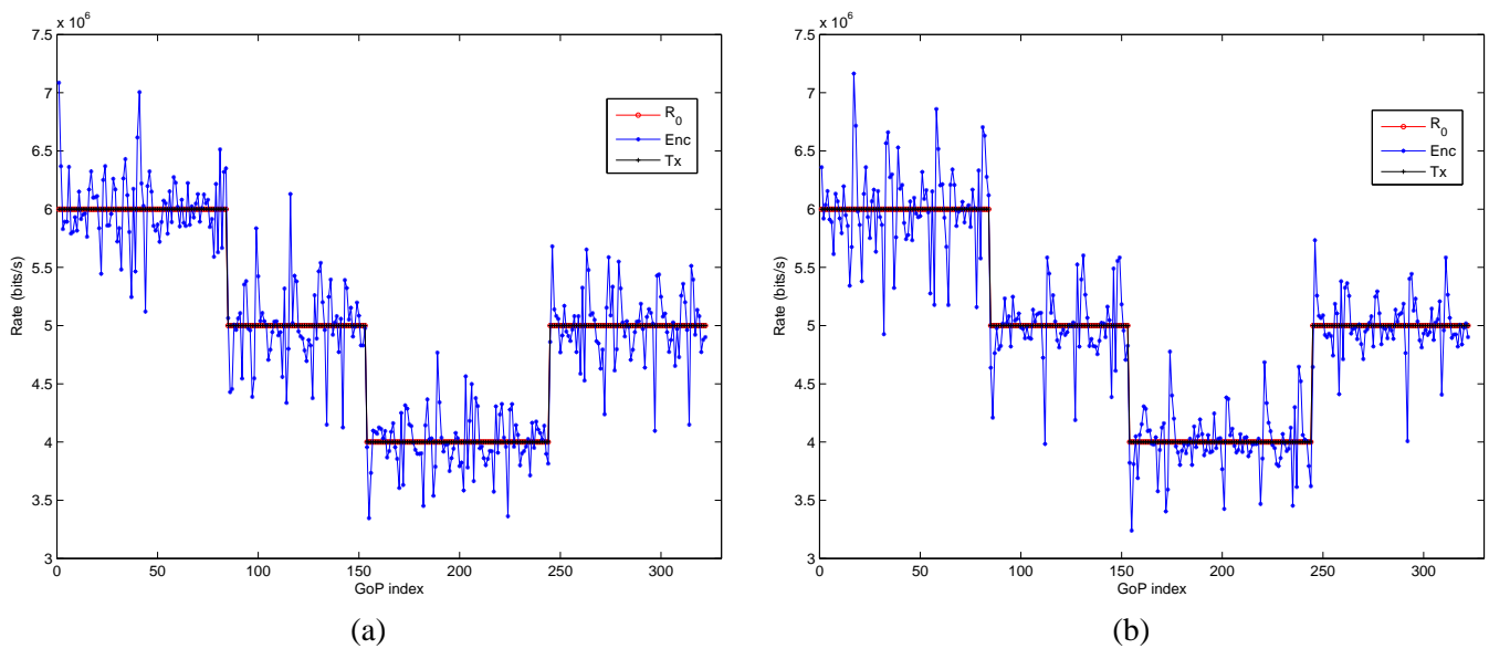
Figure 13. Total transmission rate, individual and total encoding rates for the eight multiplexed programs when W = 1 (a) and W = 2 (b)
