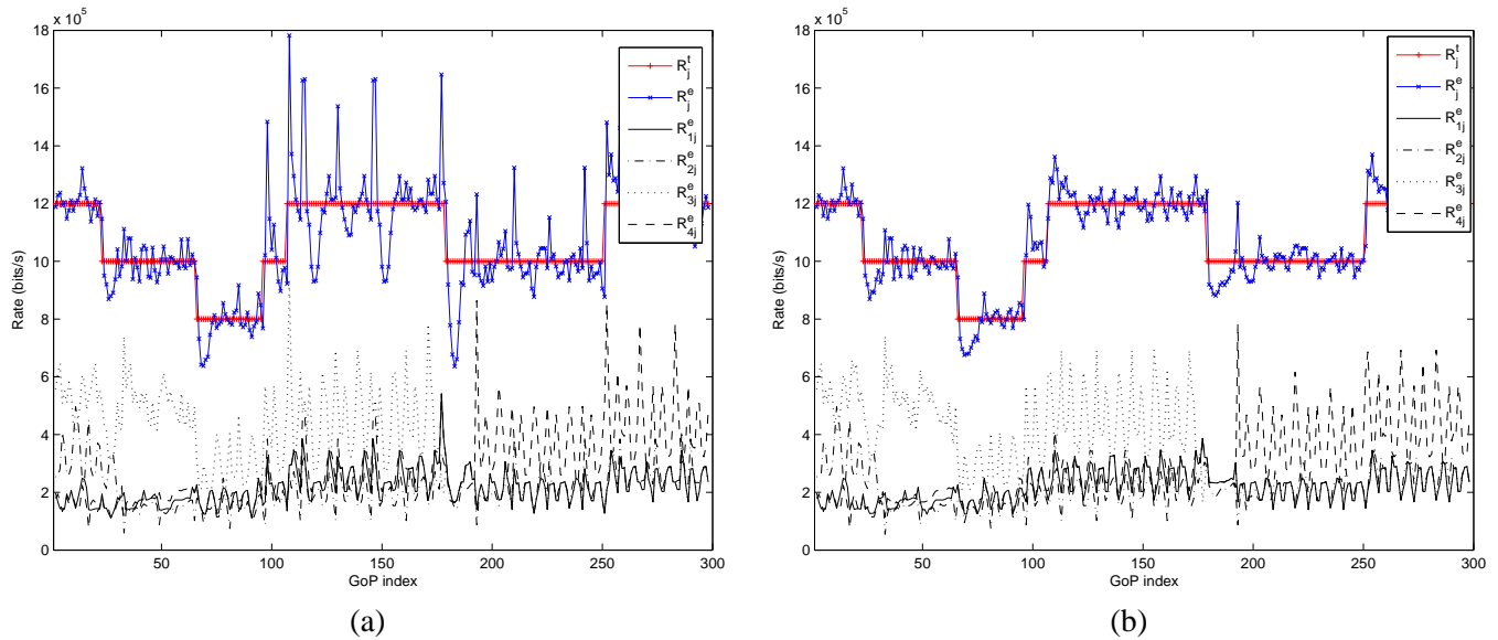
Figure 10. Evolution of the total transmission rates as well as individual and total encoding rates for the four multiplexed programs when W = 2 (a) and W = 4 (b) with variable channel rate
