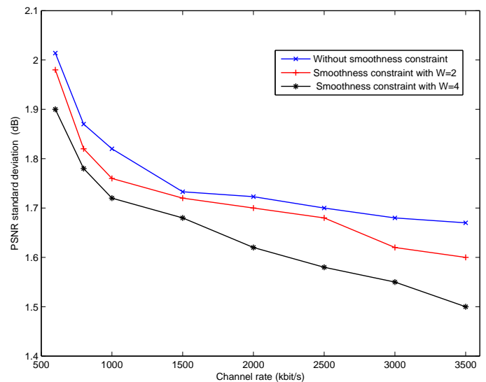
Figure 7. Standard deviation of the PSNR without imposing any smoothness constraint W = 1 , with smoothness constraint when W = 2 and W = 4 for different channel rates
