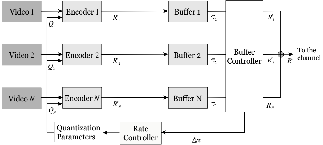
Figure 1. Proposed closed-loop statistical multiplexing system
