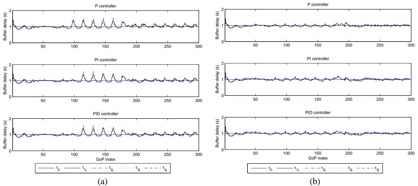
Figure 8. Buffering delay evolution of the 4 multiplexed programs using P, PI, and PID controller with W = 2 (a) and W = 4 (b) in the encoder control process with constant channel rate
