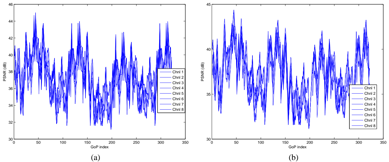
Figure 14. PSNR of the eight multiplexed programs when W = 1 (a) and W = 2 (b)
