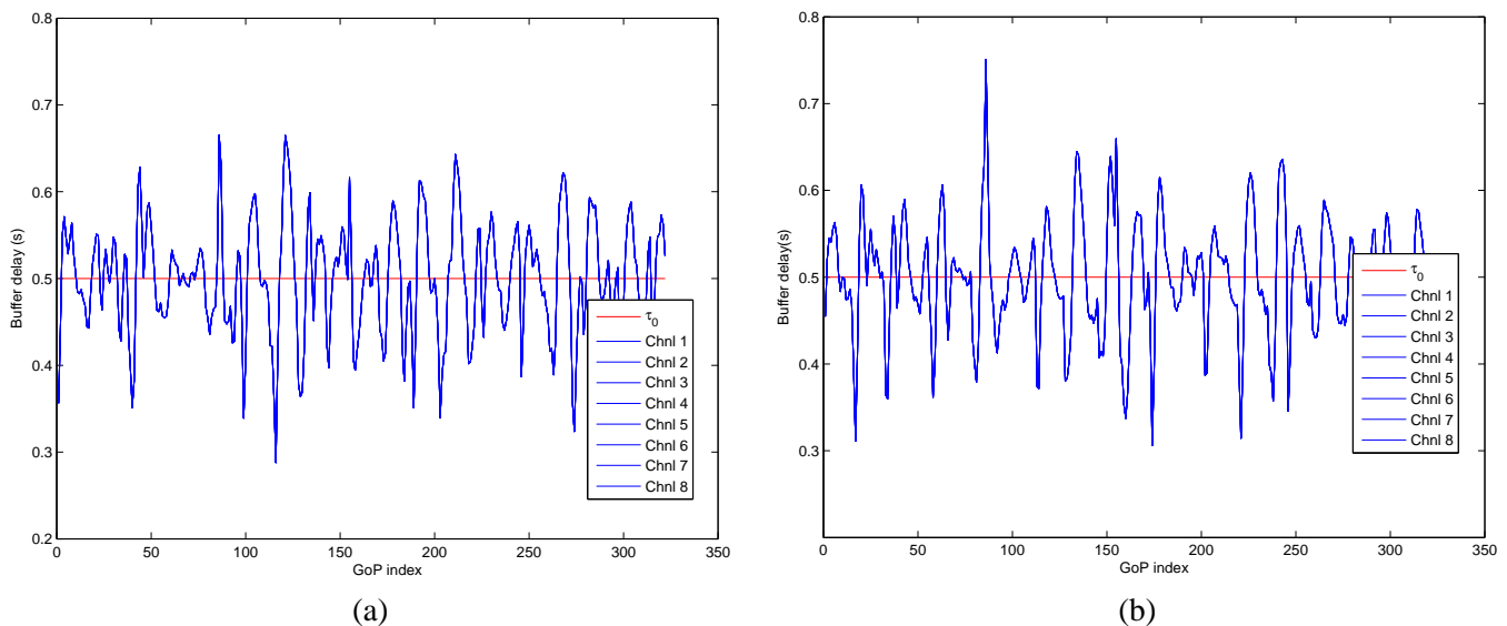
Figure 16. Buffering delay evolution of the eight multiplexed programs with W = 1 (a) and W = 2 (b)
