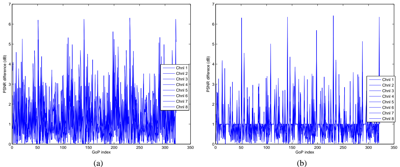
Figure 15. PSNR differences of the eight multiplexed programs when W = 1 (a) and W = 2 (b)
