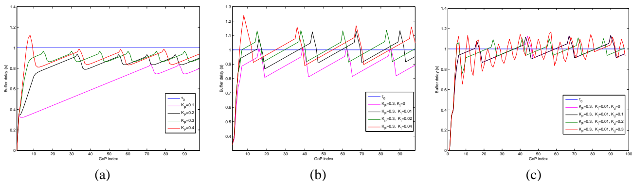
Figure 9. Tuning of the parameters of the PID controller: (a) P controller, (b) PI controller, (c) PID controller
