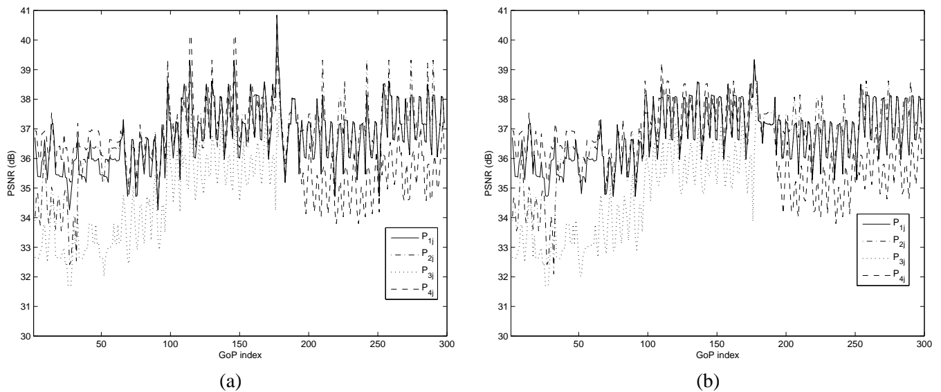
Figure 11. Evolution of the PSNR of the four multiplexed programs when W = 2 (a) and W = 4 (b) with variable channel rate
