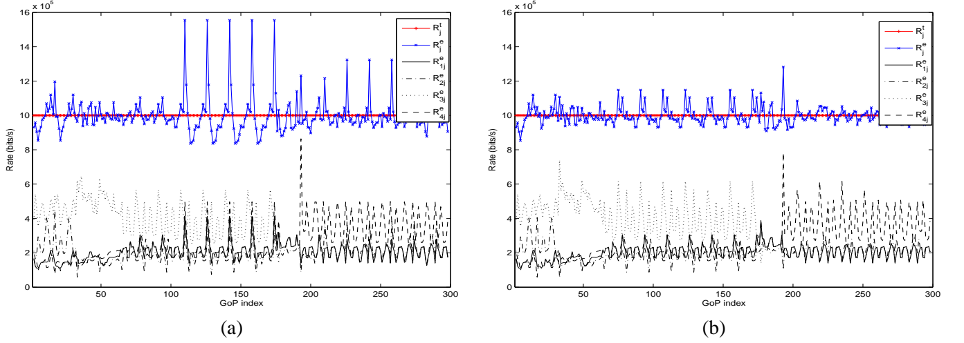
Figure 4. Evolution of the total transmission rates as well as individual and total encoding rates for the four multiplexed programs when W = 2 (a) and W = 4 (b)
