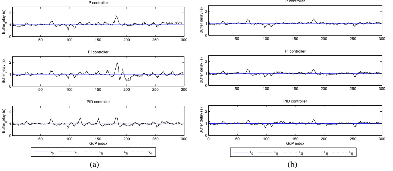
Figure 12. Buffering delay evolution of the four multiplexed programs using P, PI, and PID controller with W = 2 (a) and W = 4 (b) in the encoder control process with variable channel rate
