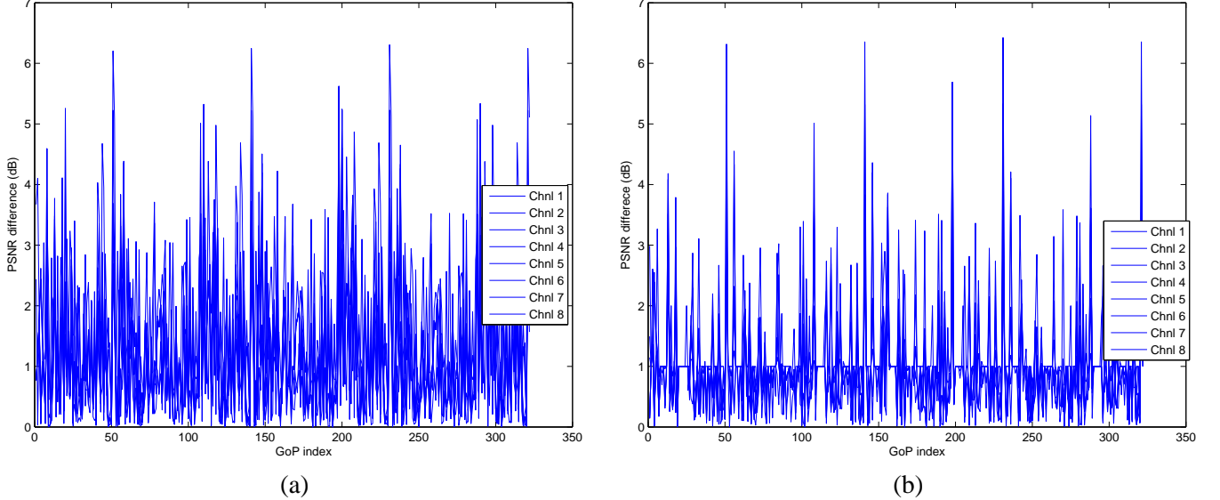
Figure 15. PSNR differences of the eight multiplexed programs when W = 1 (a) and W = 2 (b)
