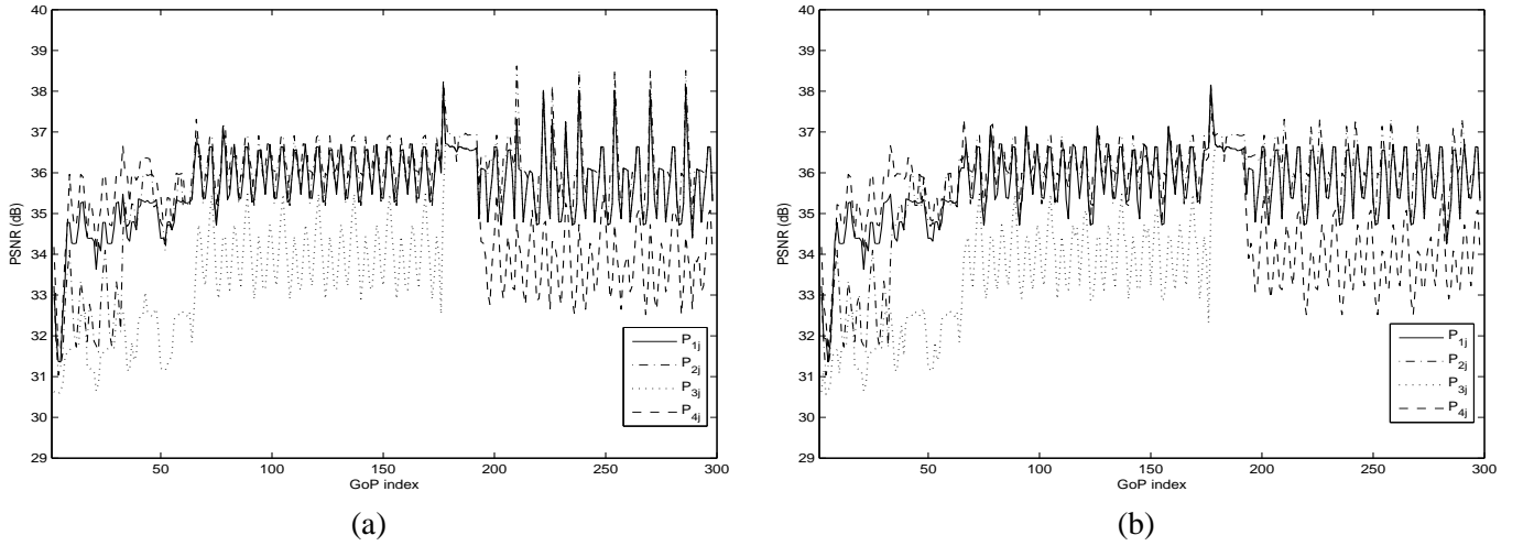
Figure 5. Evolution of the PSNR of the four multiplexed programs when W = 2 (a) and W = 4 (b)
