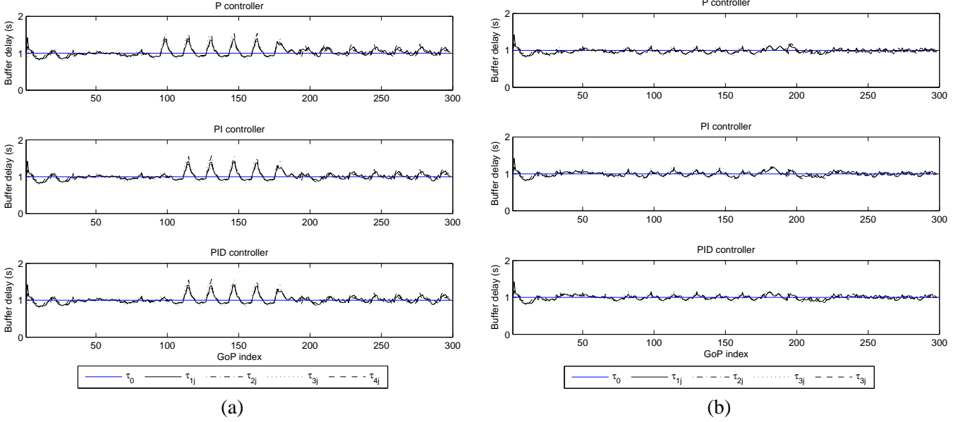
Figure 8. Buffering delay evolution of the 4 multiplexed programs using P, PI, and PID controller with W = 2 (a) and W = 4 (b) in the encoder control process with constant channel rate
