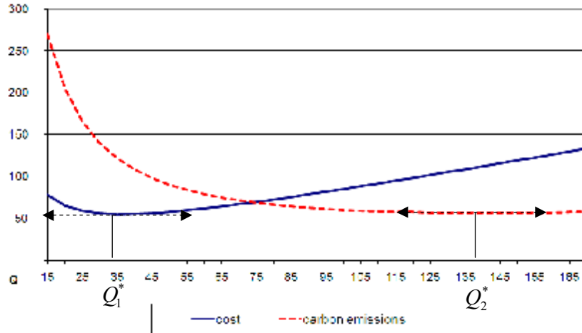
Figure 2 Cost and carbon emissions in function of the batch size
