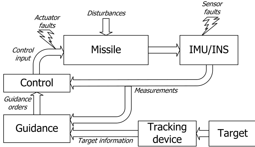
Figure 3: GNC scheme
