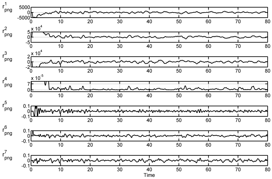
Figure 18: Wind and no fault - residuals for the PNG law
