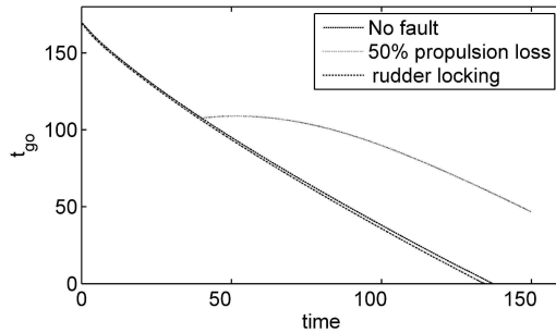
Figure 6: Estimation of t_{go} in different fault conditions
