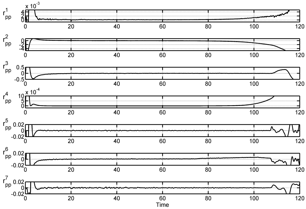
Figure 17: Scenario 8 - residuals for the PP law
