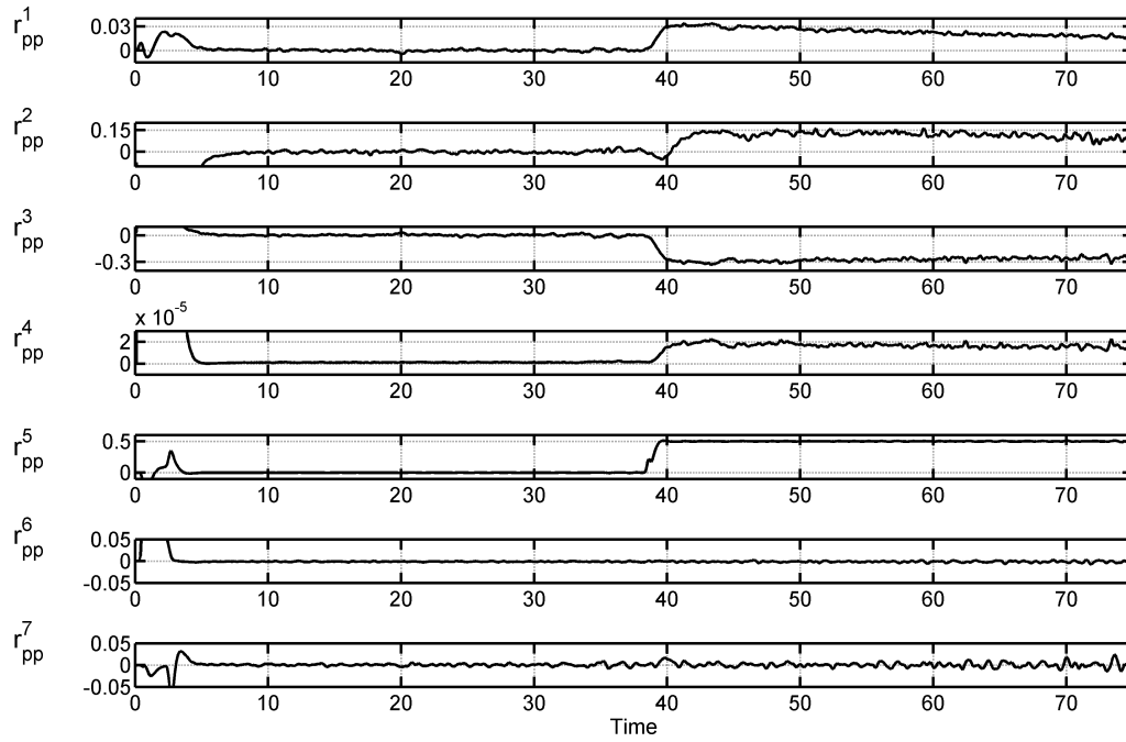
Figure 13: Scenario 4 - residuals for the PP law
