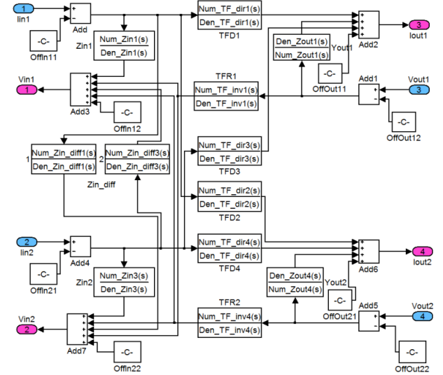
Figure 6 : Simulink macro-model for the differential design
