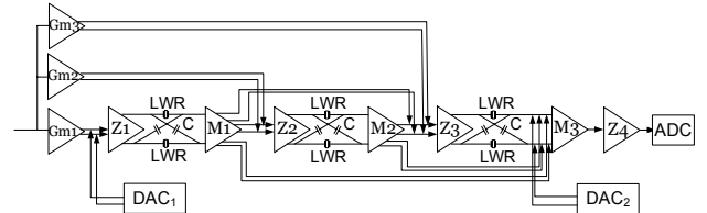
Figure 3 : Sixth-order Sigma-Delta modulator
