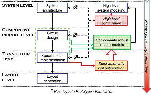
Figure 1: Refined top-down design methodology
