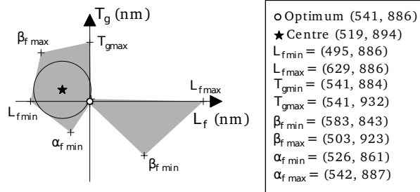
Figure 5: Tolerance map of L_f and T_g . The variation ranges of \alpha_f = L_f + T_g and \beta_f = L_f/\alpha_f define a polygon (grey) of allowed (L_f, T_g) couples for the design. The centre of the incircle (★) enhances the robustness of the optimum point (○).
