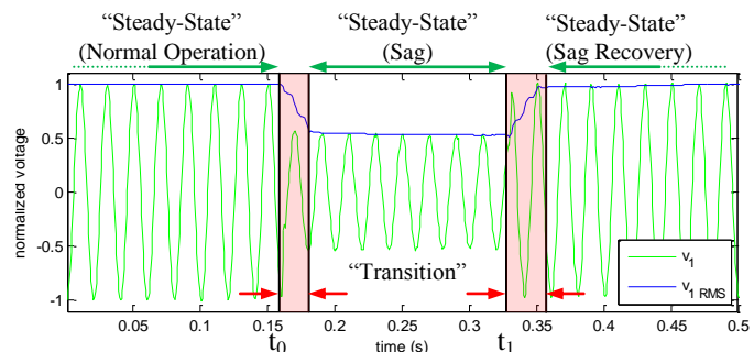
Fig. 1. Splitting of a disturbance into steady-state and transition segments. Appearance of a line-to-line fault at t_0 = 160 ms, recovering at t_1 = 330 ms. Shaded areas indicate the transition segments of the disturbance.
