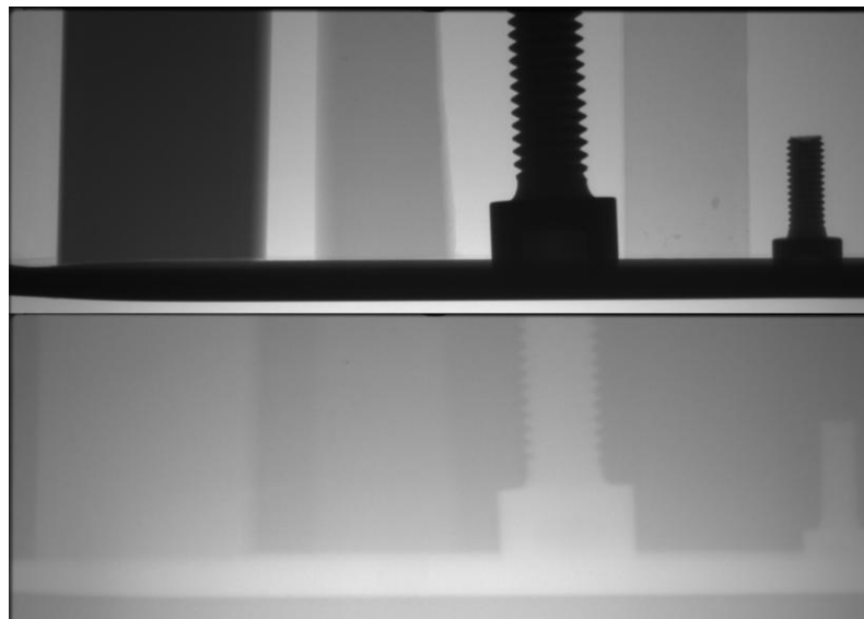
Figure 2 : luminous ghosts resulting form protection from irradiation (top: static image 15s at 160kV/350 \mu A, bottom: flat field after 15hrs at 160kV/350 \mu A).
