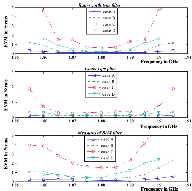
Figure 8: EVM in function of the (co-)simulated filter
