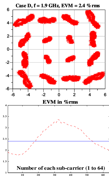
Figure 7 : Constellation and EVM (all sub-carriers)
