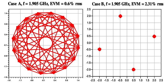
Figure 5: Constellations at 1.905 GHz, case A and B
