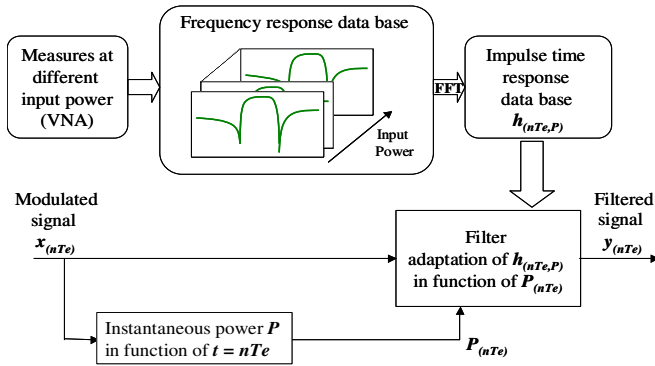
Figure 9 : Principle of the algorithm
