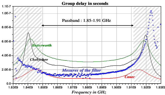
Figure 4: Group delay of the different filter types
