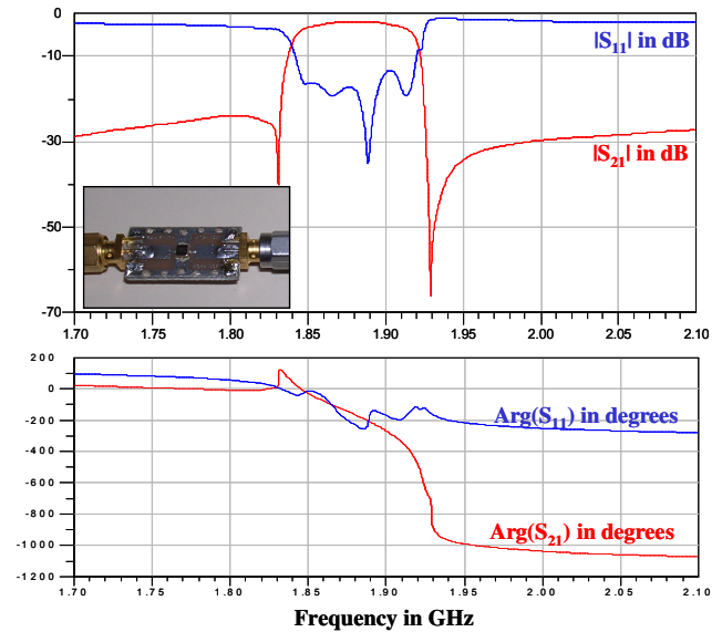
Figure 1: Measurements of a BAW ACPF7001 filter.
