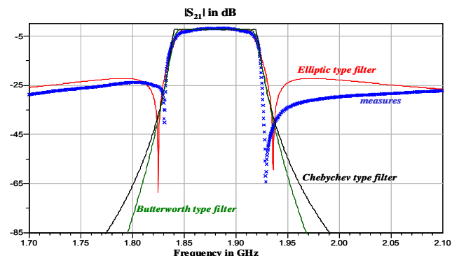
Figure 1: Measurements of a BAW ACPF7001 filter.
