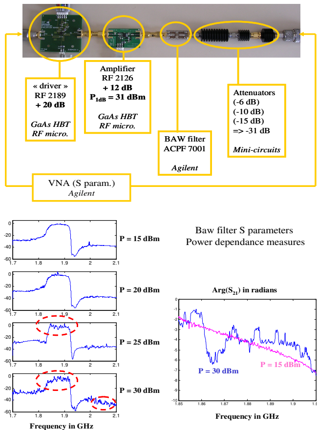
Figure 10: Measures (top) and extraction of S21
