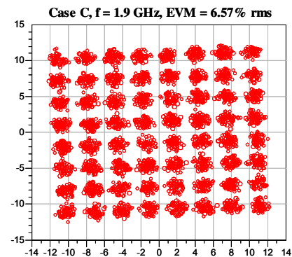
Figure 6: Constellation at 1.9 GHz, case C
