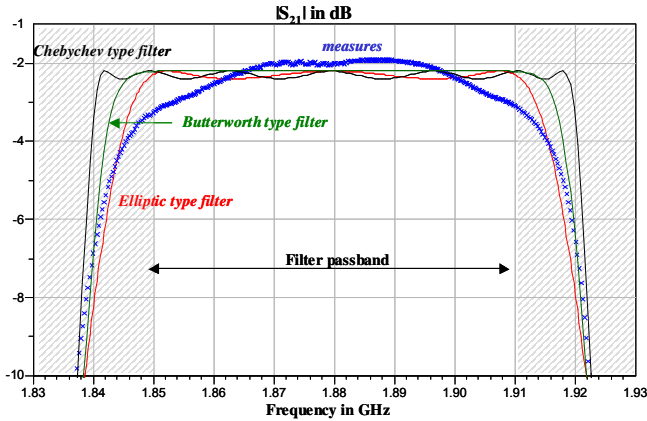
Figure 3: 20 \cdot \log_{10}|S_{21}| of the different filter types
