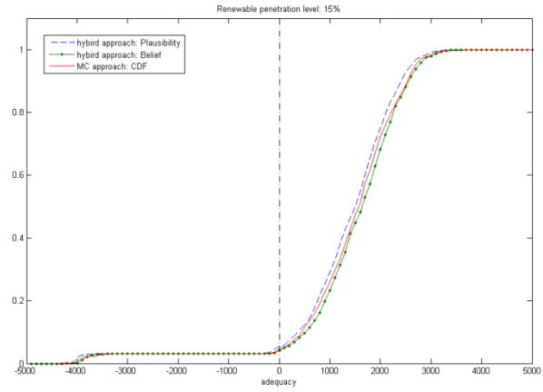
Fig 6. Comparison of joint propagation and pure probabilistic approaches at renewable penetration level of 15%
