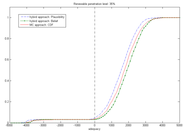
Fig 8. Comparison of joint propagation and pure probabilistic approaches at renewable penetration level of 35%
