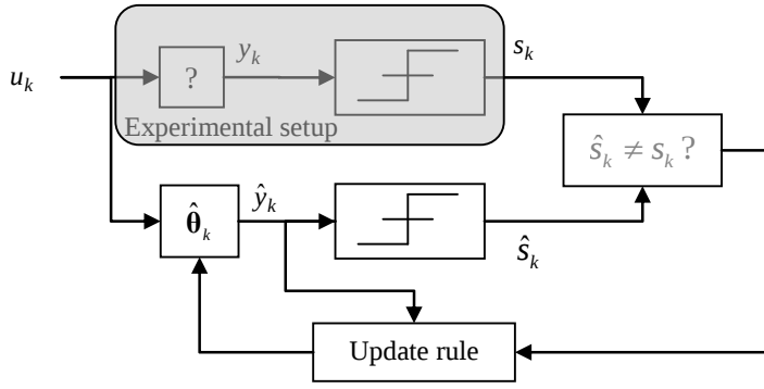
Fig. 1 - Block diagram of the LIMBO method. The measured output s_k are \pm 1 . The inputs u_k may also be binary.
