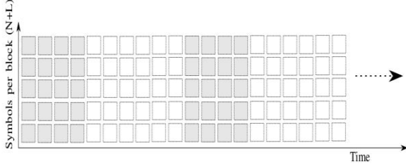
Figure 5 Output of the Pilot insertion block, the matrix P is denoted in gray.
