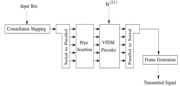
Figure 4 VFDM TX block diagram.
