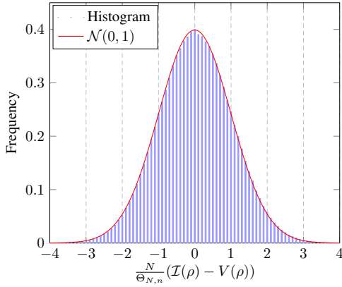
Fig. 4. Histogram of the random variable \frac{N}{\sigma_{N,n}}(\mathcal{I}(\rho) - V(\rho)) versus the Gaussian \mathcal{N}(0, 1) law. SNR = 5 dB, n = 9 .
