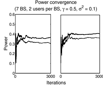
Fig. 6. Power convergence for Systems S4 and S5 (H2 Network)
