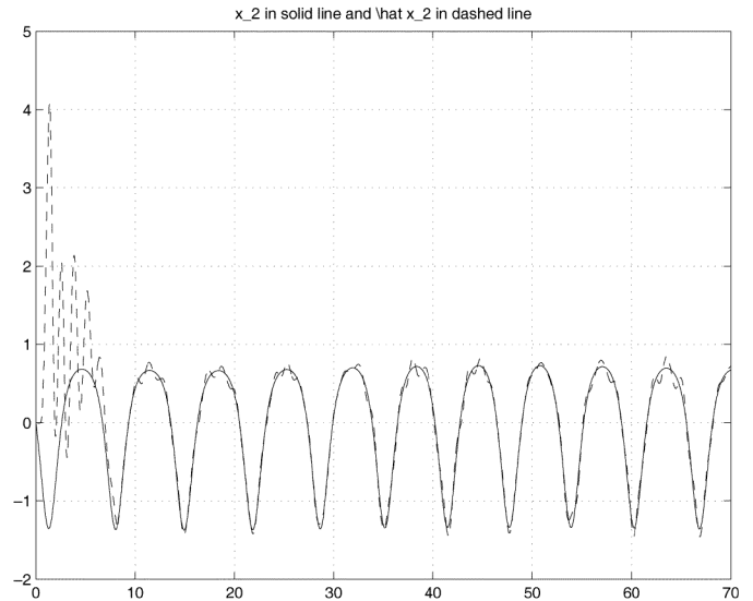
Fig. 5. Evolution of the second state for \tau = 0.5 s with a cascade of two observers.
