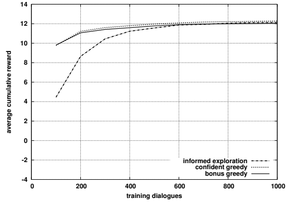
Figure 1: Performance of the trained policies (greedy setting). To compute the average reward, each 100 dialogues, 100 policies were trained and tested in a greedy way 1000 times each.
