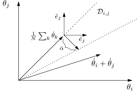
Fig. 1. Geometric interpretation of desynchronization
