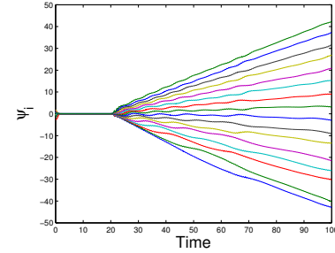
Fig. 3. Evolution of the grounded dynamics of (17) for large natural frequencies when a proportional mean-field feedback with gain \gamma = -k_0 is switched on at time t = 20 .
