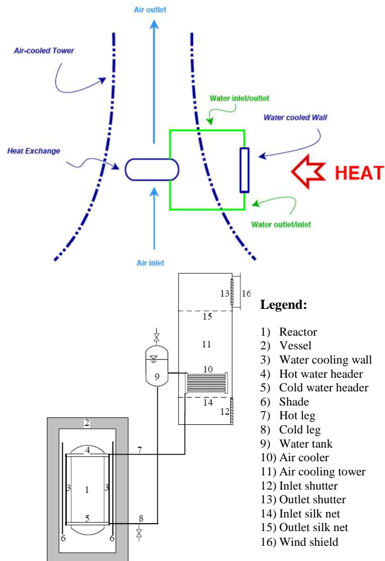
Figure 3 Schematics of 1 train of the RHRs in the HTR-PM [Zhao et al., 2008]
