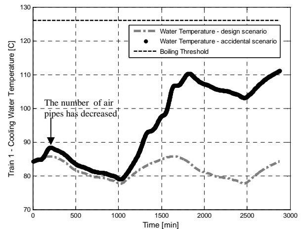
Figure 6 Evolution of the outlet water temperature in RHR train 1.
