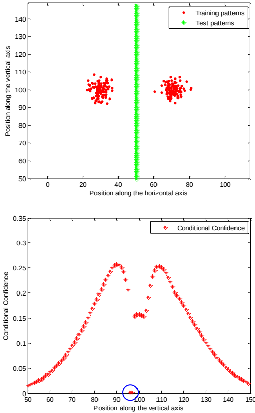
Figure 5 Case study 4: degree of confidence for patterns equally distant from two clusters (ECM with a small radius value).
