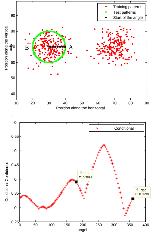
Figure 3 Case study 2: variation of the degree of confidence in the reconstruction depending on the presence of other clusters.
