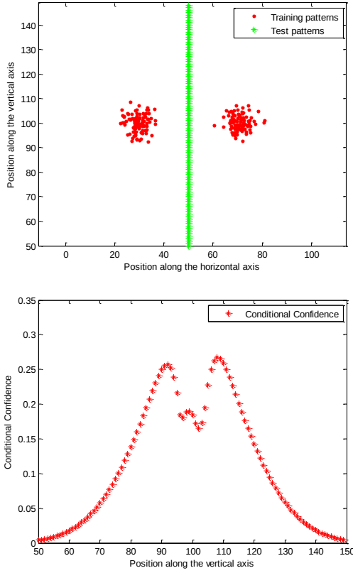
Figure 4 Case study 3: degree of confidence for patterns equally distant from two clusters (ECM with a large radius value).
