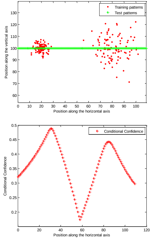
Figure 6 Case study 5: variation of the degree of confidence in function of the cluster density.
