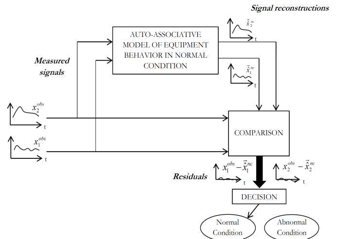
Figure 2. Condition monitoring scheme.
