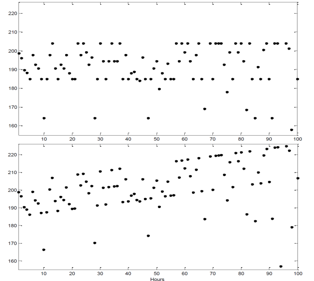
Figure 7. Time evolution of signal 10d in normal condition during 100 consecutive hours (top); time evolution of signal 10d in abnormal condition, linearly drifted by 0.7% of the standard deviation.
