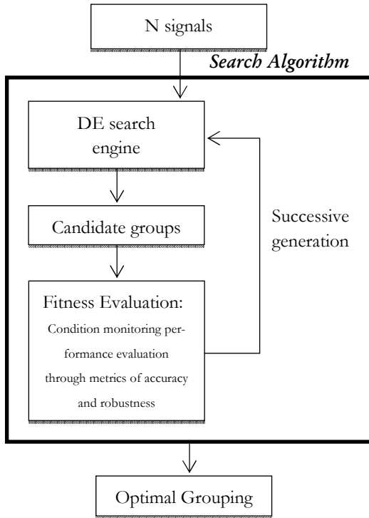
Figure 1. Wrapper approach for optimal signals grouping.
