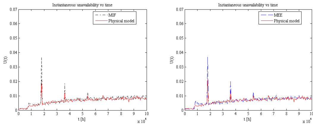
Figure 15: instantaneous component unavailability during the time horizon, with an inspection interval of 18000 h.
