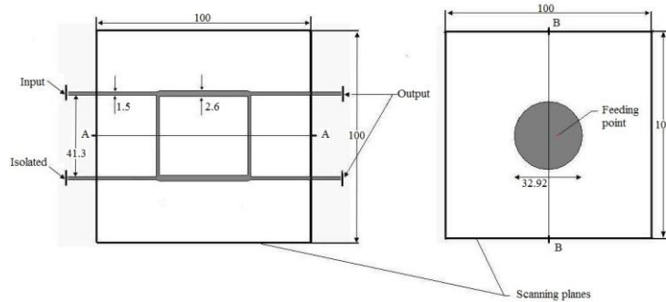
Figure 3. Upper view and description of the used devices under test. (left) quadrature hybrid coupler, (right) circular patch antenna.
