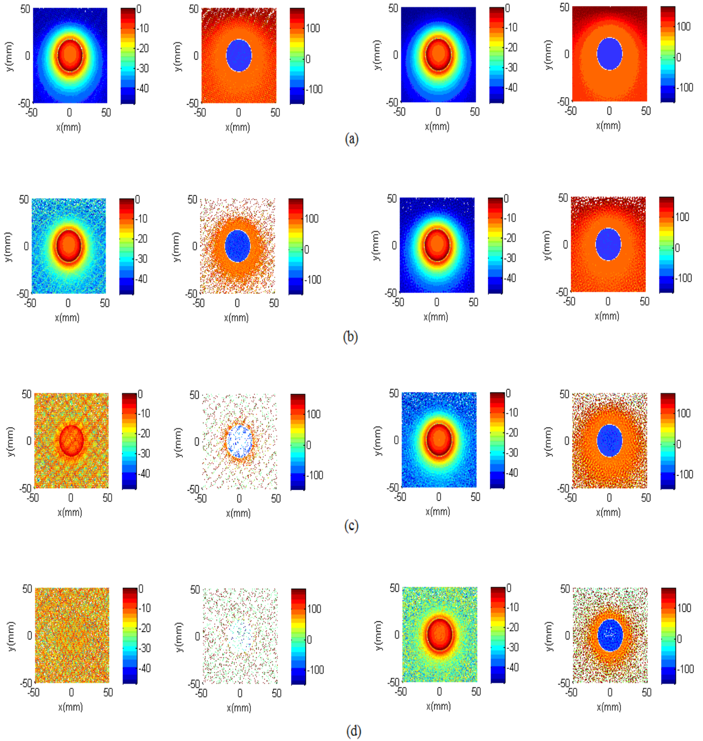
Figure 4. The normalized amplitude [dBV/m] and phase [deg] of the normal electric field radiated by the patch antenna calculated by DIF (left) and CLSF (right), for different added noise levels, a: -100dB, b: -80dB, c: -60dB and d: -40 dB
