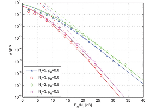
Fig. 1. Setup: N_t = 8 , \Omega_0 = 1 , and m_0 = 2.5 . Markers: Monte Carlo simulation. Solid lines: numerical integration in (1). Dashed lines: high SNR framework in (14) and (15).
