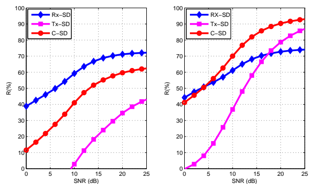
Fig. 3. Computational complexity against the SNR. N_t = N_r = 4 , (left) M = 8 ; (right) M = 64 .
