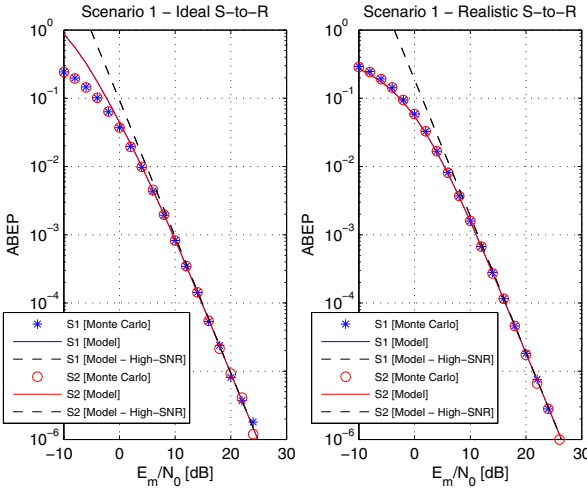
Fig. 2. ABEP against E_m/N_0 for Scenario 1 ( \sigma_0^2 = 1 ).
