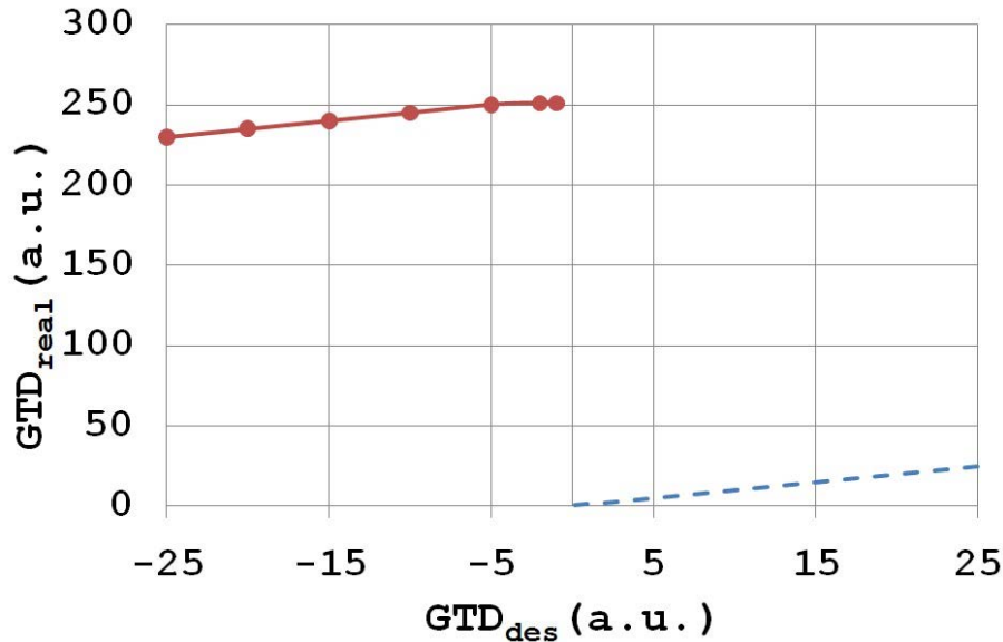
Figure 7. Real (anti-aliased) normalized GTD ( \text{GTD}_{\text{real}} ) as a function of desired normalized GTD ( \text{GTD}_{\text{des}} ) for a grating synthesized by the DLP method. Reflectivity is considered to be maximal for every simulation point. The values of GTD are normalized so that each unit corresponds to a phase derivative d\phi_{\text{BG}}/d\lambda of 1rad/nm.
