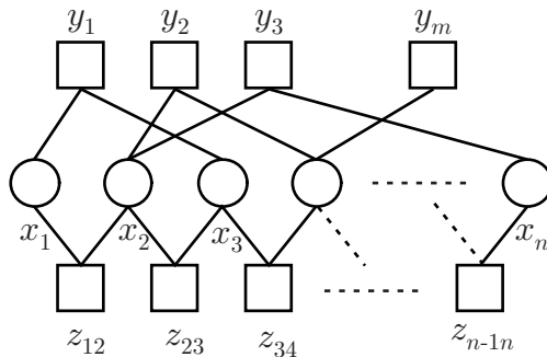
Figure 4: Bipartite graph associated with the joint source-network coding problem
