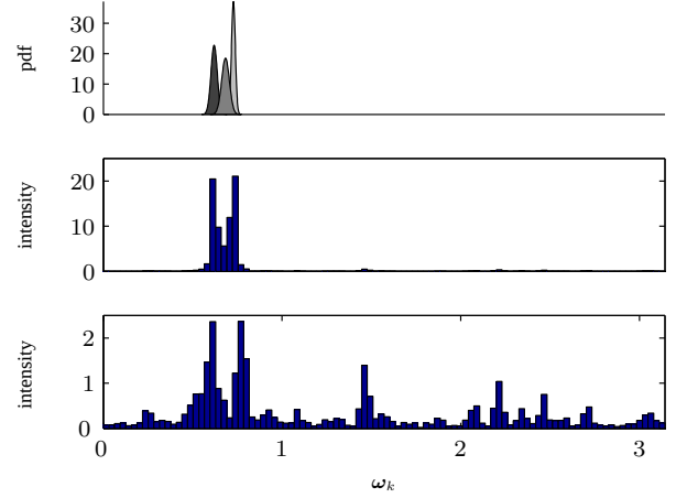
Fig. 4: The pdf of fitted Gaussian components (top), the histogram intensity of all radial frequencies samples (middle), and the histogram intensity of the allocated samples to the Poisson point process component (bottom).
