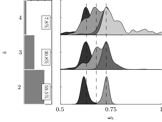
Fig. 1: Posteriors of k (left) and sorted radial frequencies, \omega_k , given k (right). The true number of components is three. The vertical dashed lines in the right figure locate the true radial frequencies.
