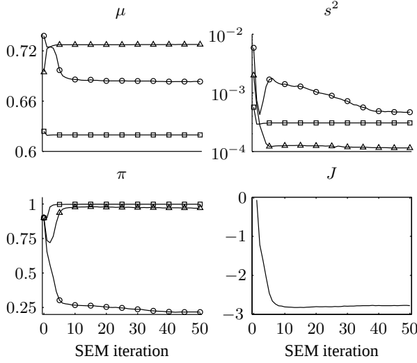
Fig. 3: Performance of the proposed summarizing algorithm on the sinusoid detection example. There are three Gaussian components in the model.
