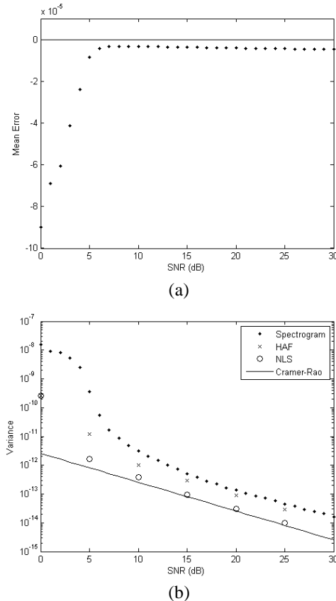
Figure 5 : Mean error (a) and variance (b) of the frequency rate using the spectrogram and NLS estimators
