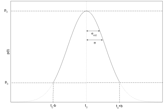
Figure 2 : p(t)
