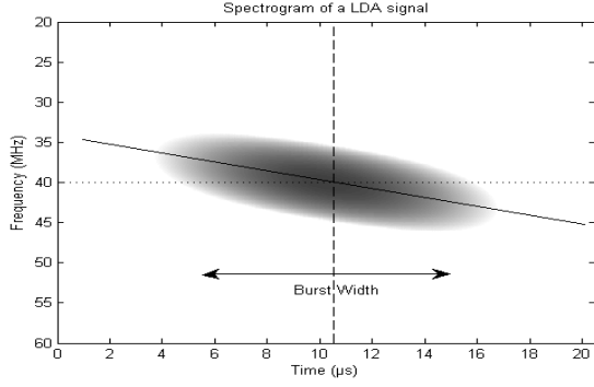
Figure 1: Spectrogram of an LDA signal: f_D is the dotted line, t_0 the dashed line and \beta the slope of the solid line.
