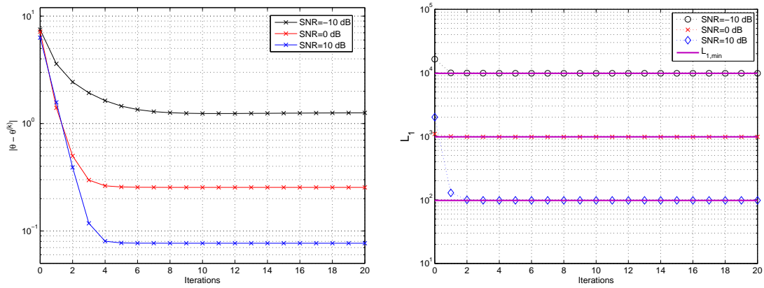
Fig. 8 RMSE of the source at 10^\circ for the nonregular array \mathbf{d} = [0, 1.32, 3.03, 5] \frac{\lambda}{2} , at SNR = -10, 0 and 10 dB, ray \mathbf{d} = [0, 1.32, 3.03, 5] \frac{\lambda}{2} , at SNR = -10, 0 and 10 dB, DOA = [-5^\circ, 10^\circ] . Fig. 9 Negative log-likelihood for the nonregular array \mathbf{d} = [0, 1.32, 3.03, 5] \frac{\lambda}{2} , at SNR = -10, 0 and 10 dB, DOA = [-5^\circ, 10^\circ] .
