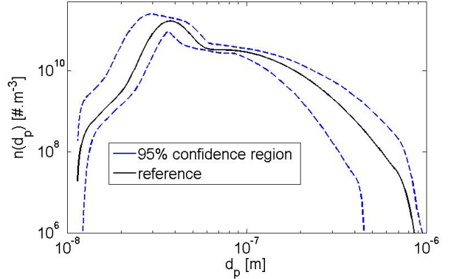
Fig. 4. 95% Confidence region on an atmospheric aerosol size distribution
