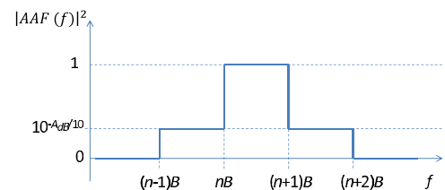
Fig. 1. Anti-aliasing filter magnitude modelling
