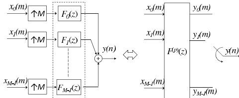
Fig. 4. HFB synthesis filter bank and its polyphase representation
