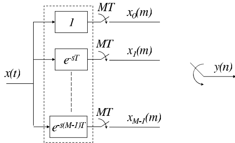
Fig. 2. TI-ADC model
