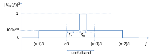
Fig. 5. Magnitude response of the analysis filter of channel m
