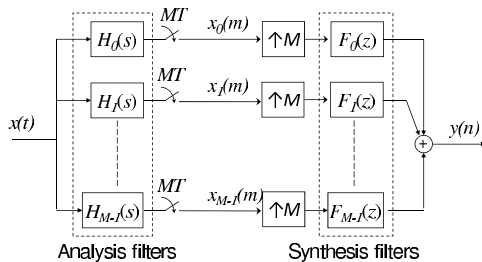
Fig. 3. HFB model
