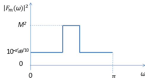
Fig. 6. Magnitude response of the synthesis filter of channel m , corresponding to the analysis filter bank given in Fig. 5
