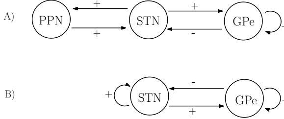
Fig. 2. Two different Schematic diagrams: Diagram A with three neuron populations (two excitatories and one inhibitory) and diagram B with two excitatory-inhibitory neuron populations.
