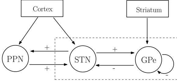
Fig. 1. Schematic diagram of three nuclei: STN, GPe and PPN.
