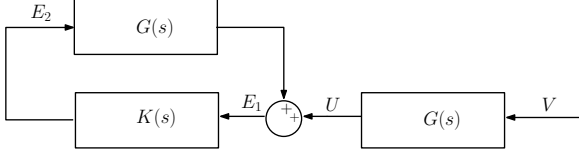
Fig. 3. Bloc diagram of the feedback system (12).
