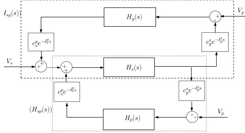
Fig. 4. Bloc diagram of the linearized system (3).
