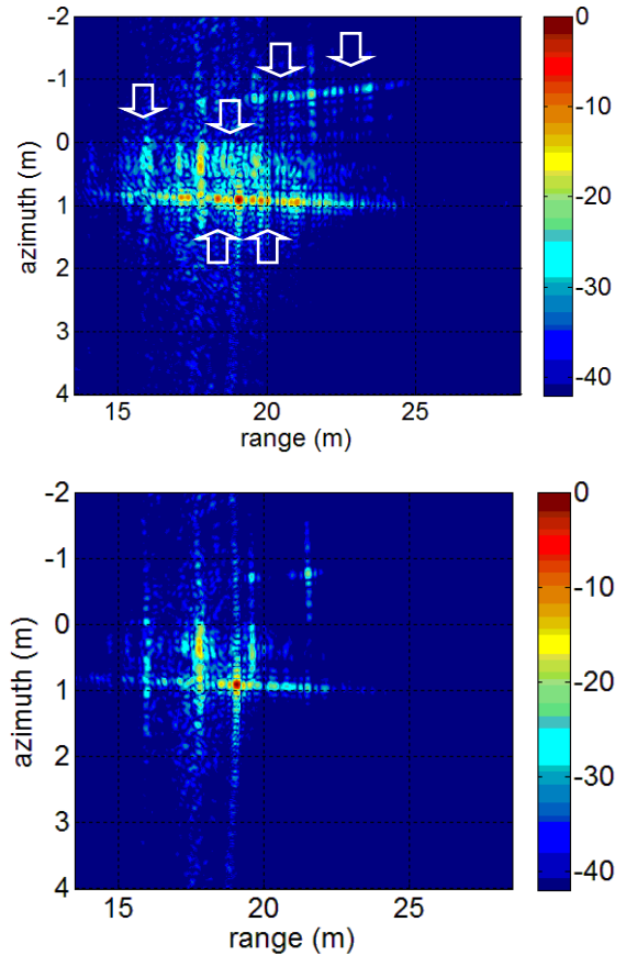
Figure 5: SAR images, top: before processing, below: after processing
