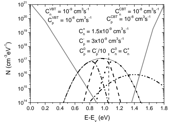
Fig. 5. DOS distributions and their capture coefficients introduced in the simulation. A defect pool model has been used to defined the DB's whose three states of charge are shown: D^+ with dotted line, D^0 in dashed line and D^- in dash dotted line. Additional acceptor states are presented in a dash-dot-dotted line.
