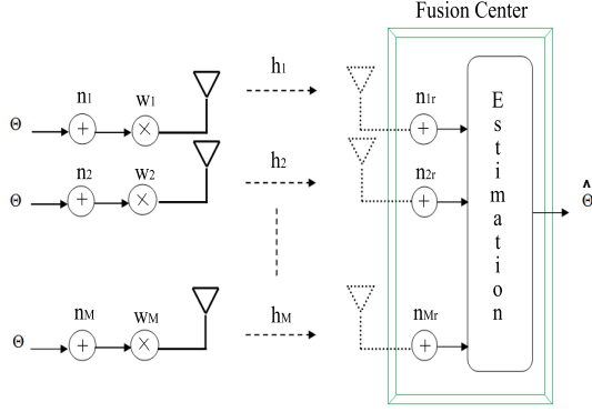
Figure 2 System model using Orthogonal channels
