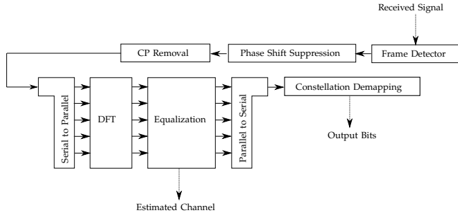
Figure 5. VFDMM RX block diagram.
