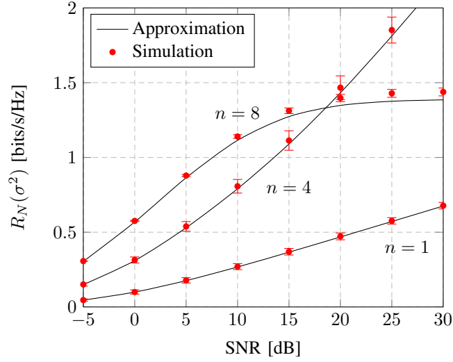
Fig. 3. Sum rate R_N(\sigma^2) at the output of the MMSE decoder for user 2 versus SNR for different numbers of transmit signatures n , N = 16 , N_i = 8 , \mathbf{P}_i = \mathbf{I}_n , \alpha = 0.5 . Error bars represent one standard deviation on each side.
