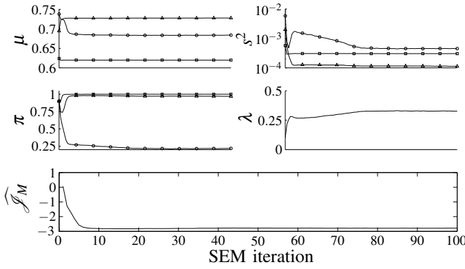
Figure 7: Evolution of the model parameters along with the criterion \widehat{J}_M defined in (8) using 100 iterations of VAPoRS with L = 3 on the RJ-MCMC output samples shown in Figure 1.
