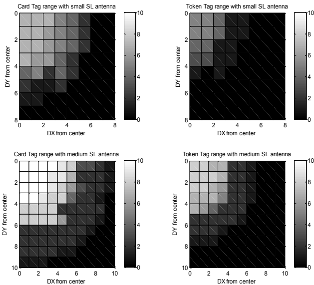
Figure 6 : Range limit for the two tags and the two SL (small/med.)
