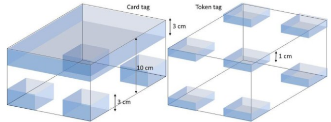
Figure 10 : ML2 volume of detection for Card and Token tags
