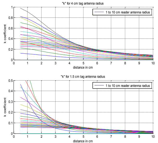
Figure 3 : “k” with equ. (2), for different tags antennas size (case A)
