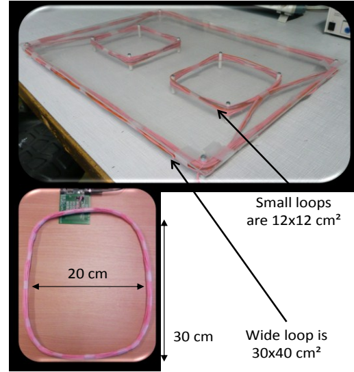
Figure 7 : ML1 (top) and wide SL (bottom)
