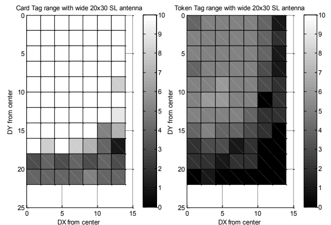
Figure 8 : SL wide range limit (2cm steps)
