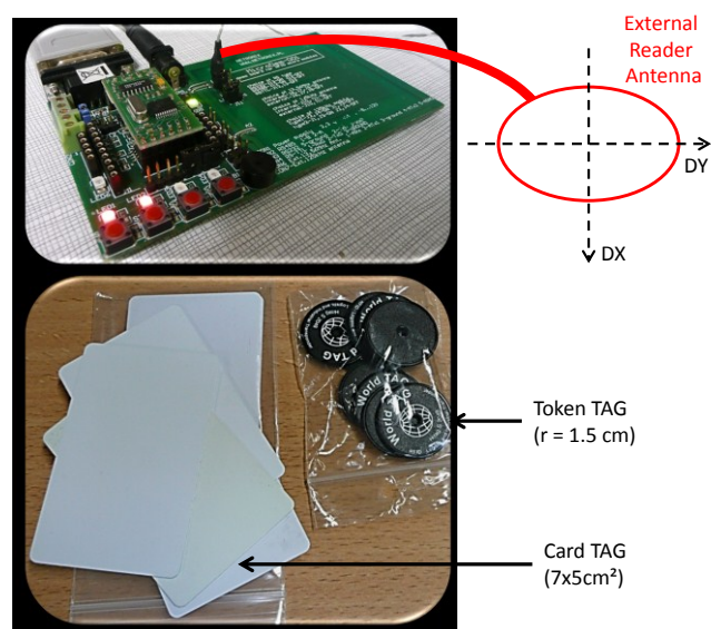
Figure 1: (Top) Netronix reader with its antenna connector (external) and the definition of DX, DY. (Bottom) Card and Token tags.
