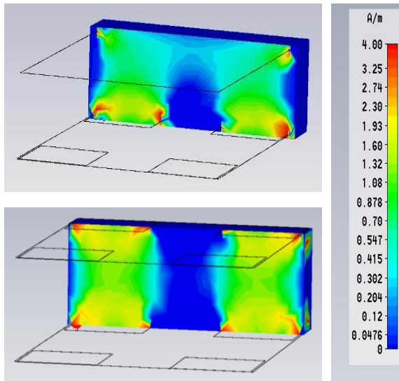
Figure 12 : H_z field for ML2 0 (top) and ML3 0 (bottom)
