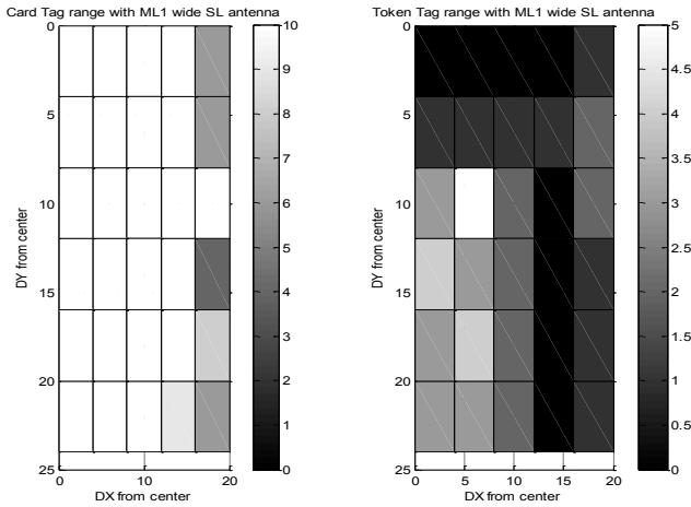
Figure 9: ML1 range limit (4cm/2cm steps)
