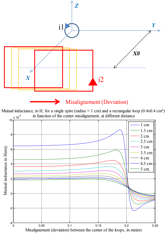
Figure 4 : Coupling between a circular loop and a rectangular wide loop at different distance (X0) and for different deviation.
