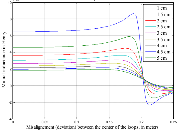
Figure 4 : Coupling between a circular loop and a rectangular wide loop at different distance (X0) and for different deviation.
